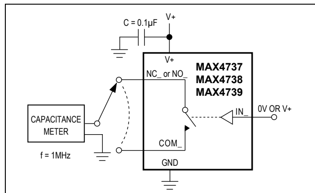
Figure 6. Channel Off-/On-Capacitance
